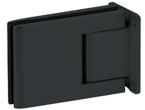
double-action hinges Agita for 8mm glass doors, black up to 60kg leaf weight / 915 mm width (left) up to 100 leaf weight kg / 1200mm width (right)
