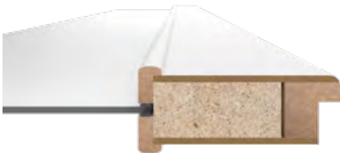
Glazing bead no 14
