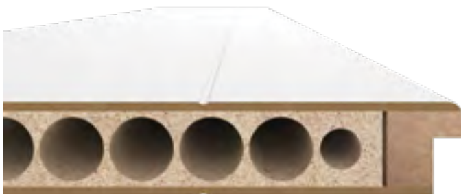
Linje cross-section, standard RSP core
